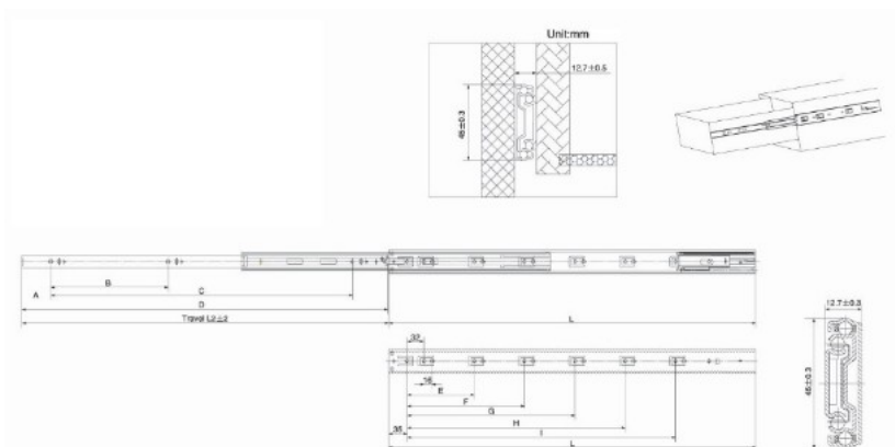
45 Series Soft-closing Dimension Table
